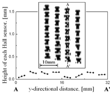
Fig. 4. Scan result of sensors array using a 3D laser displacement sensor.
