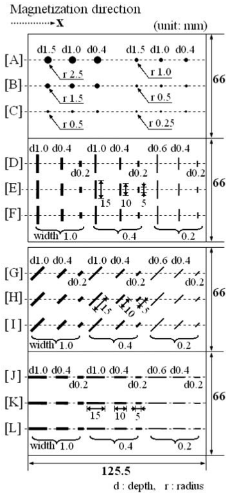
Fig. 2. Schematic graphs of cracks on each specimen.
