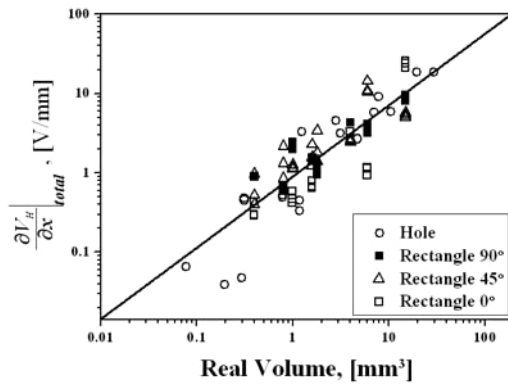
Fig. 9. Relationships between real crack volume and \partial V_H/\partial x|_{total} .
